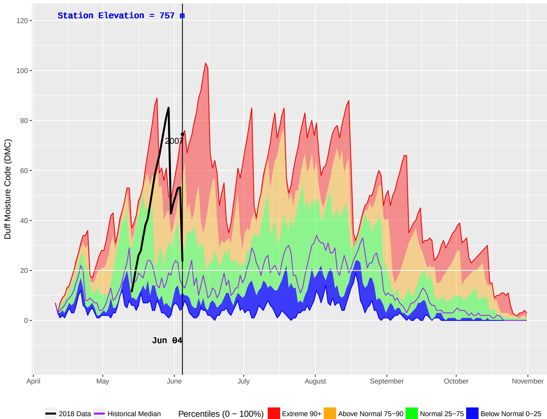
DOWNIE (905) : Historical (2005–2016) and Current (2018) Noon Duff Moisture Code (DMC)
