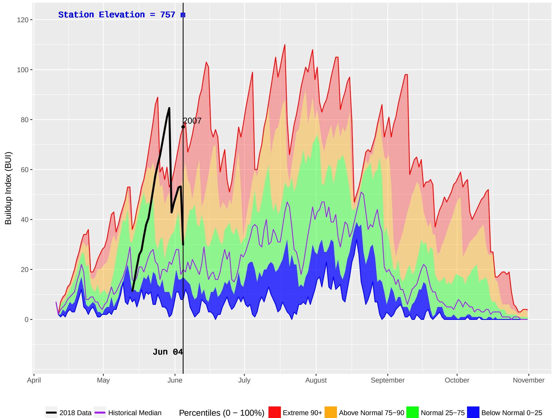
DOWNIE (905) : Historical (2005–2016) and Current (2018) Noon Buildup Index (BUI)
